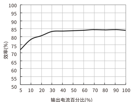
效率Vs输出负载(Vin=24V) URF2405MD-10W
